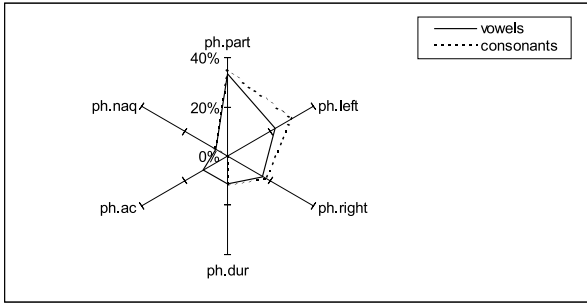
Figure 1. Relative feature rate used in PDTs, split in accordance with vowel/consonant categorization .
