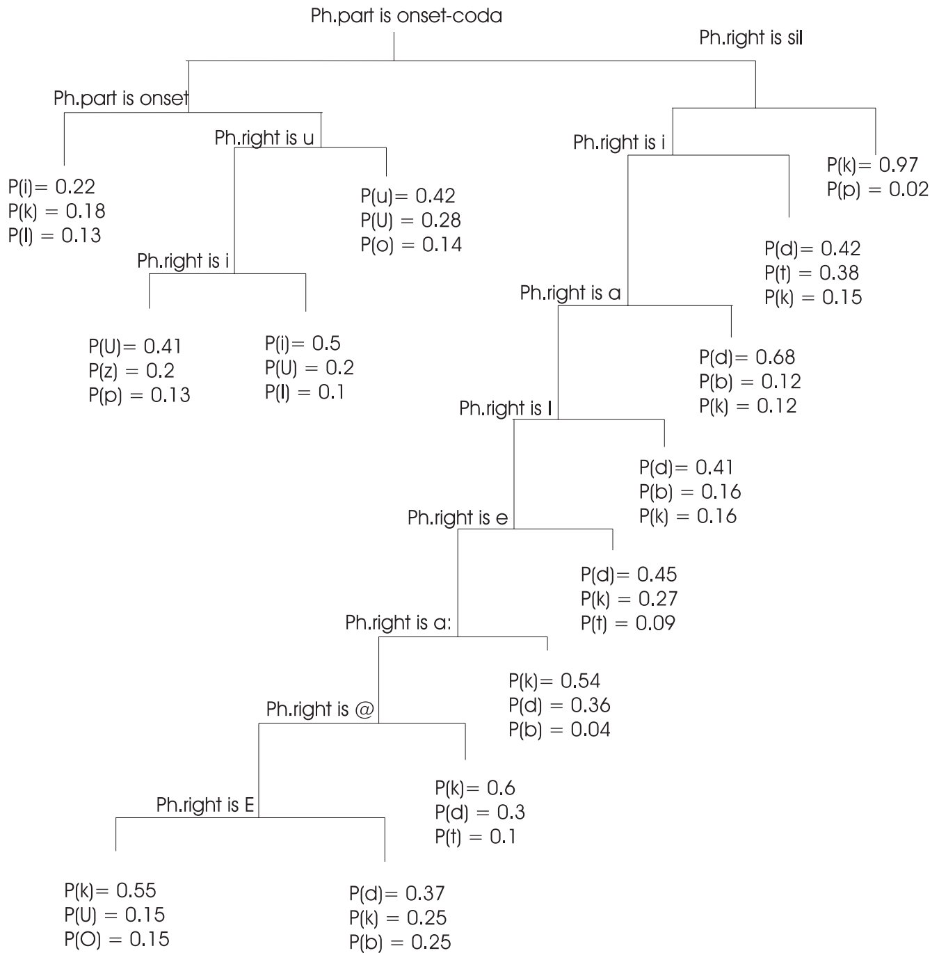
Figure 3. Decision tree of phoneme /g/. The most significant diagnostic results on the right is the misrecognition (a) of /g/ as /k/, if silence follows /g/ - the whole /g/ is misrecognized, (b) of /g/ as /d/, if /a/ follows /g/ - again the whole /g/ is affected. Looking on the left of the tree, we see an interesting impact of vowels /U/ and /I/ followed by /g/. Here the part of /g/ is decoded as /U/ or /I/ respectively. Concluding the selected main features all together, the right context of the consonant /g/ plays the most significant role in its incorrect recognition, and must be better modeled in situations, which were revealed by the diagnostic tree.
